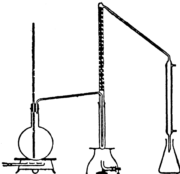
Small apparatus for the distillation of the volatile acids
