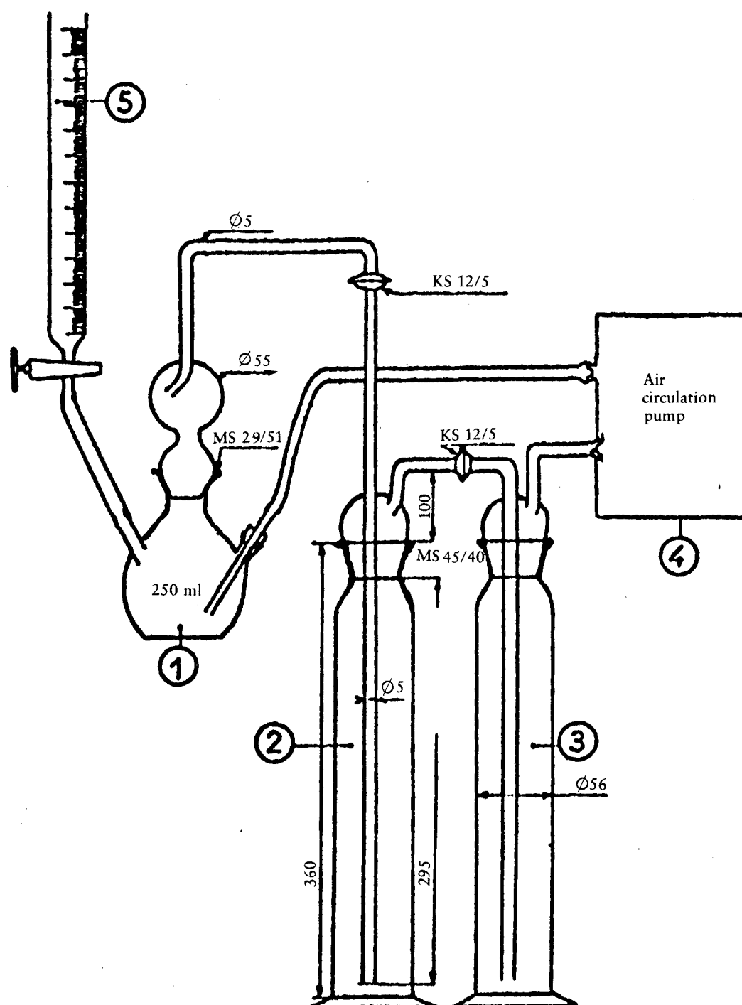
Figure 1 Apparatus for the extraction of CO 2 in closed circuit
