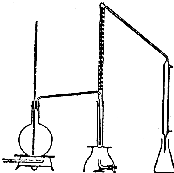
Small apparatus for the distillation of the volatile acids
