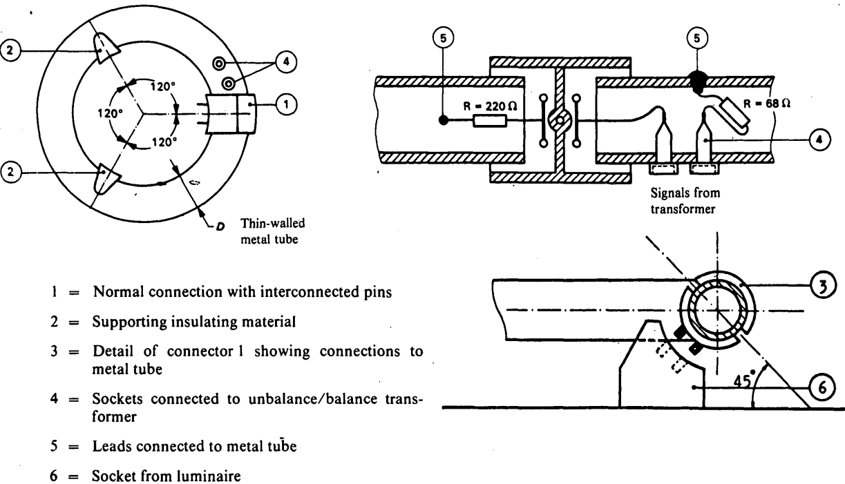
Configuration of circular dummy lamps
