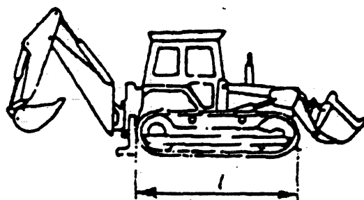
Figure 4: Excavator-loader
