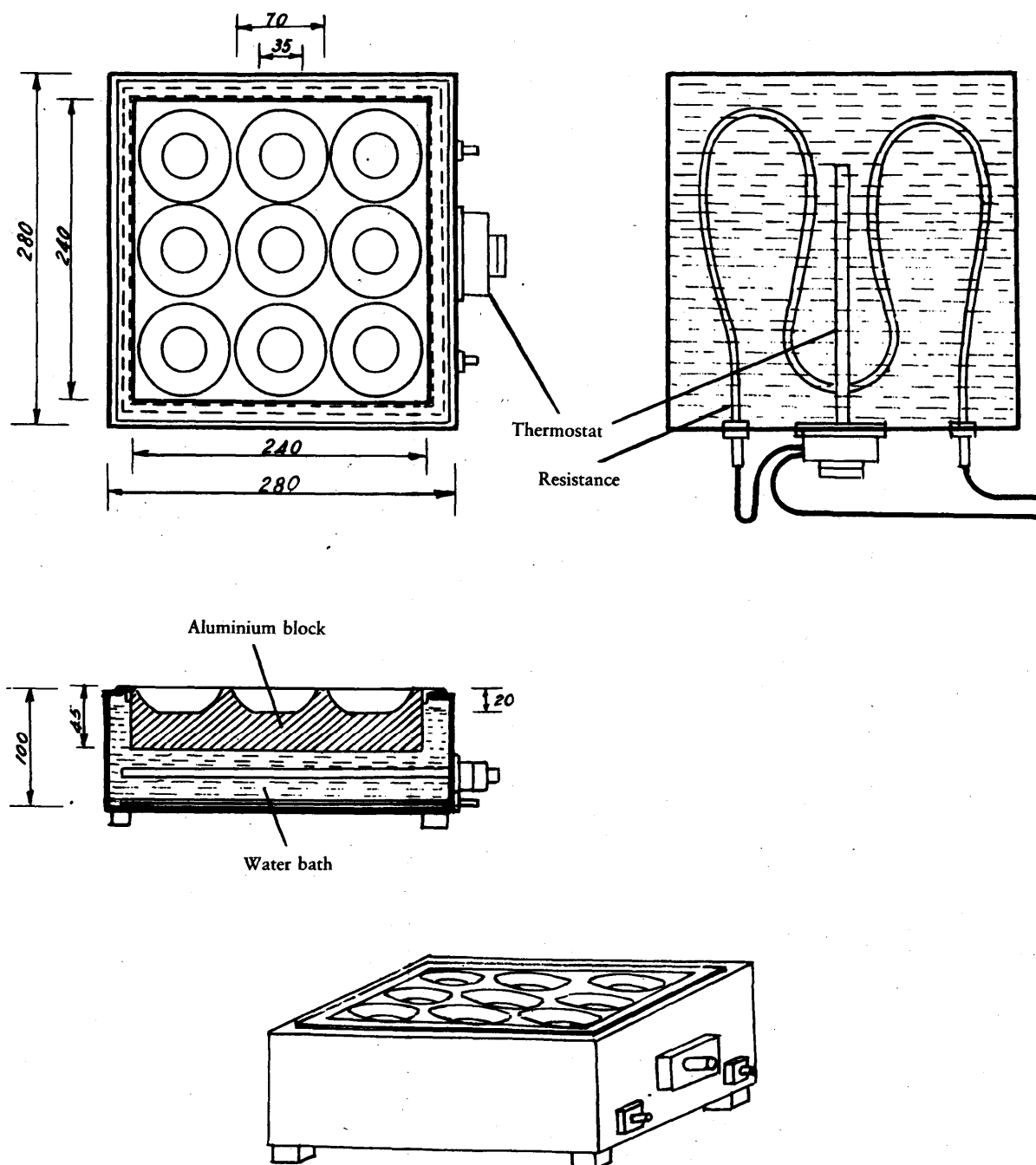
Figure 2 — Device for heating samples (dimensions in millimetres)
