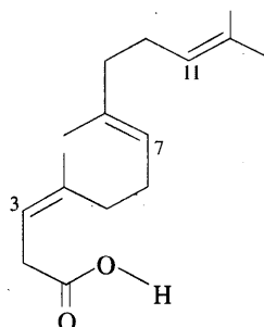
3,7-cis/trans- isomer
