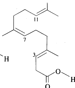
3,7-trans/ cis-isomer
