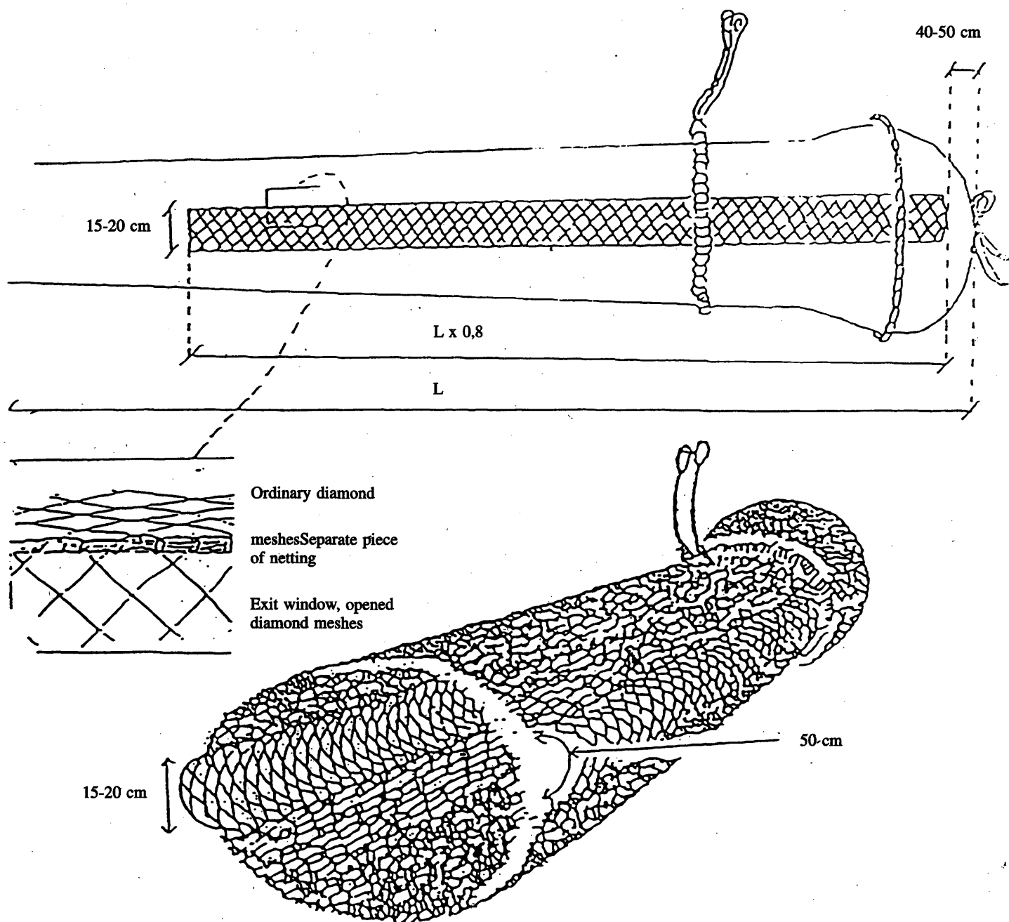
Diagram (Exit window model 1)
