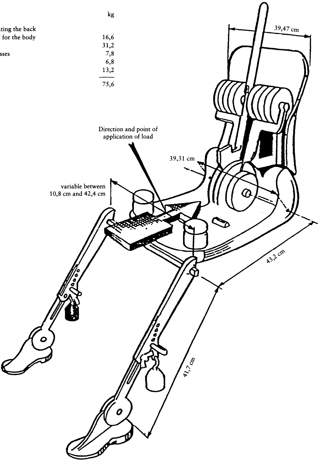
Dimensions and mass of Dummy
