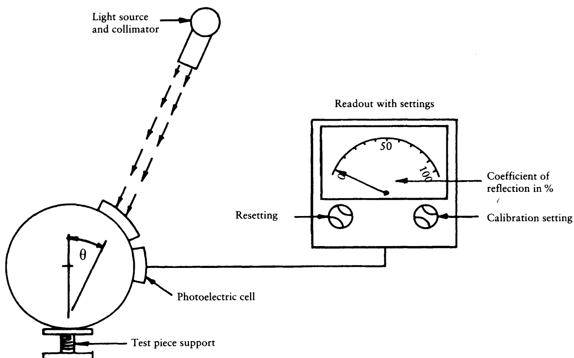
Figure 2: General layout drawing of the reflectivity measuring equipment using an Ulbricht sphere in the receiver
