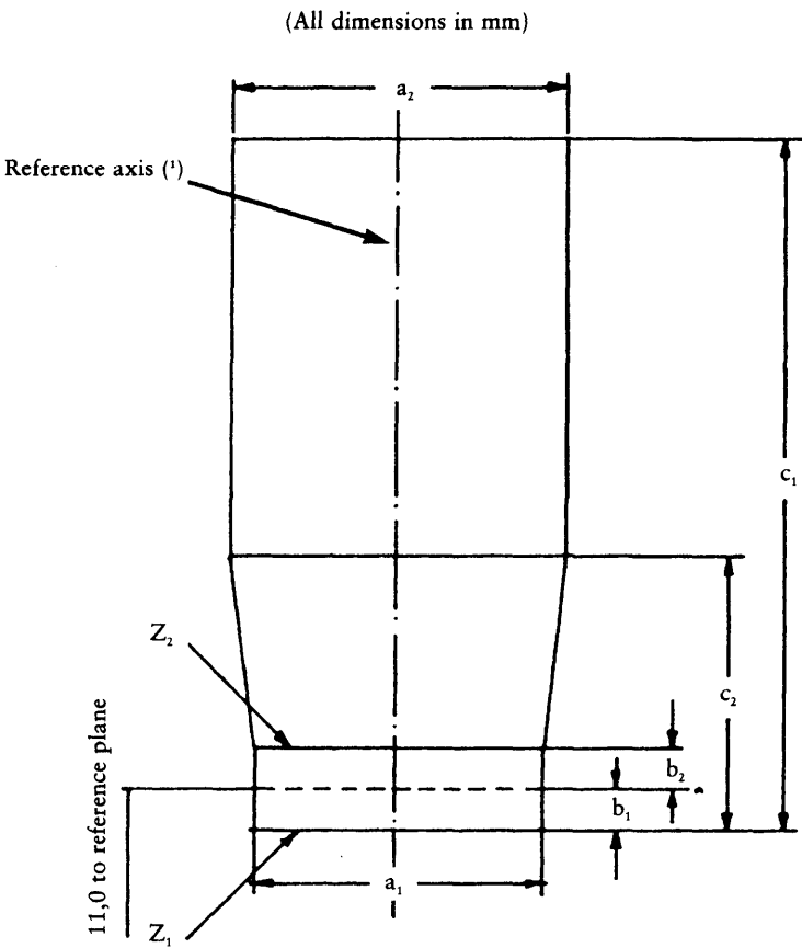
View A + B
