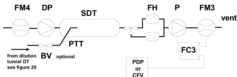
Figure 22: Double dilution system (full flow system only)
