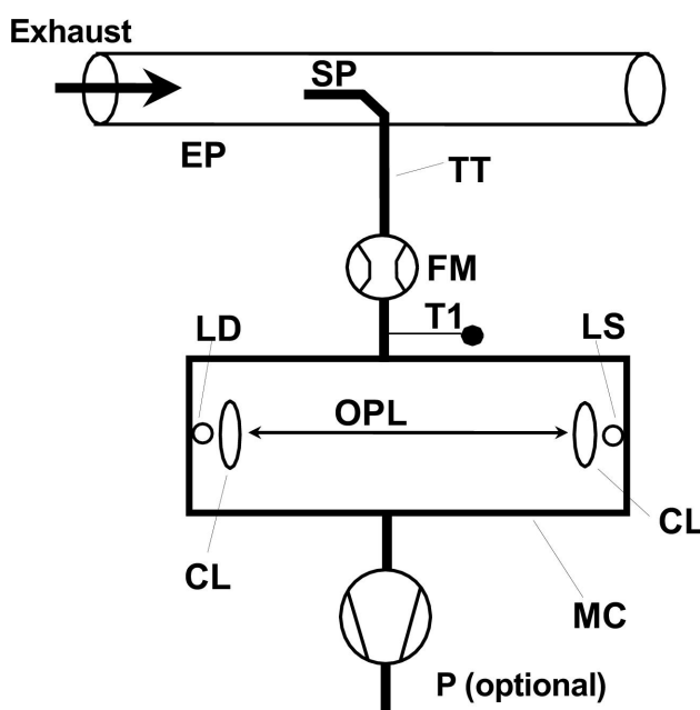
Figure 24: Partial flow opacimeter
