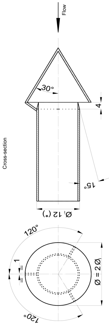
Figure 5/2 Particulate sampling probe configuration
