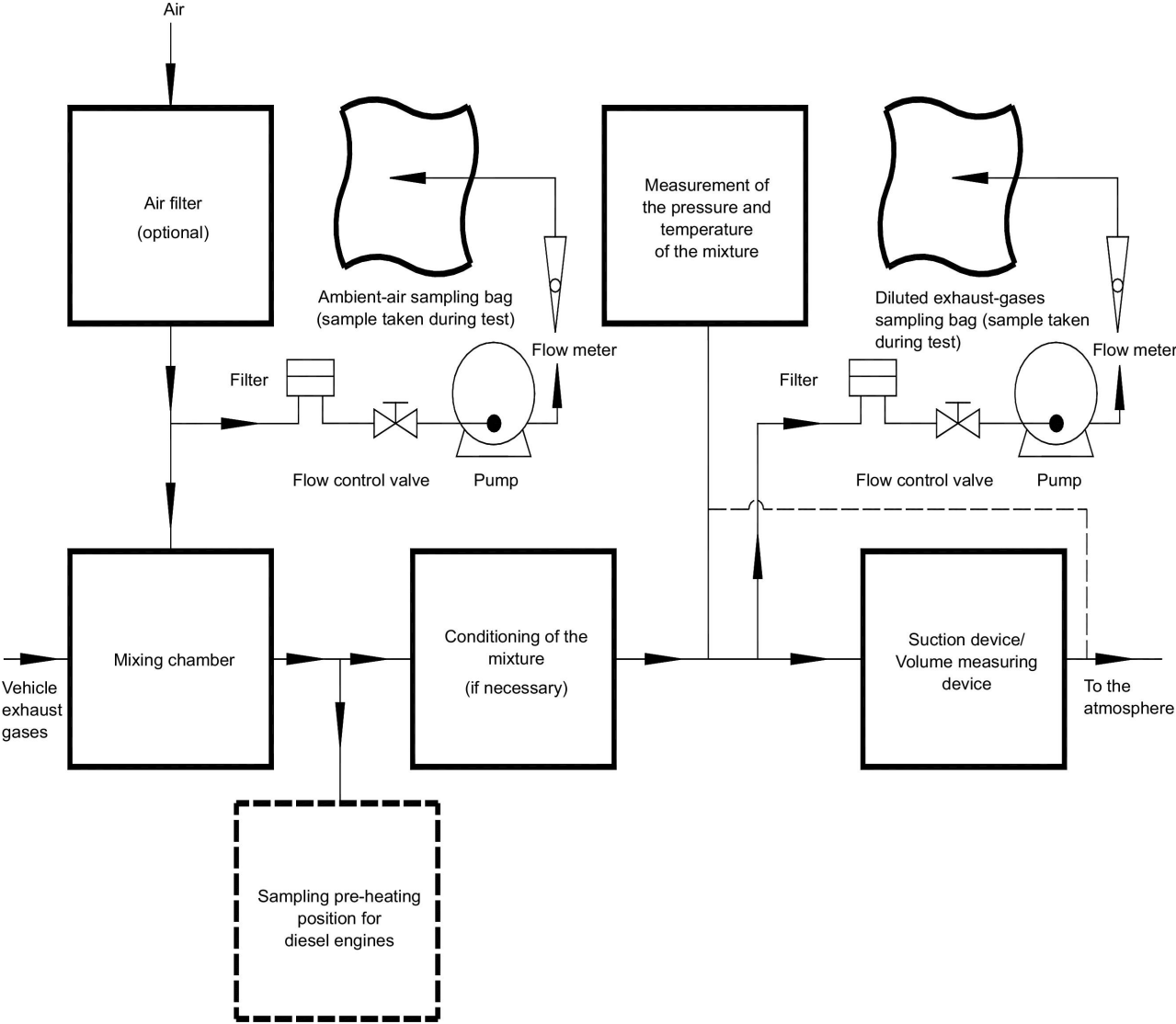
Figure 5/1 Diagram of a variable-dilution system for measuring exhaust gas emissions
