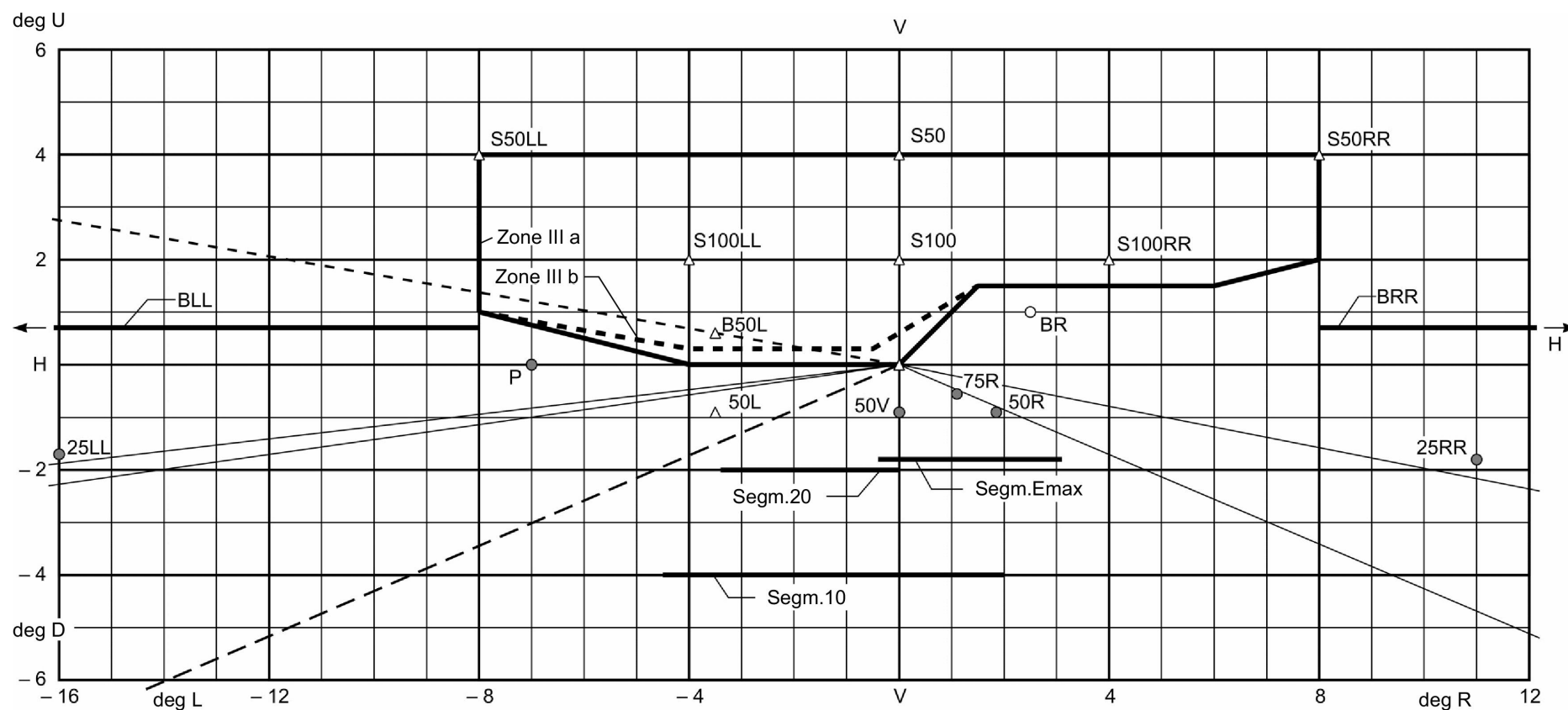
Figure 1: Angular positions of passing beam photometric requirements (indicated for right-hand traffic)
