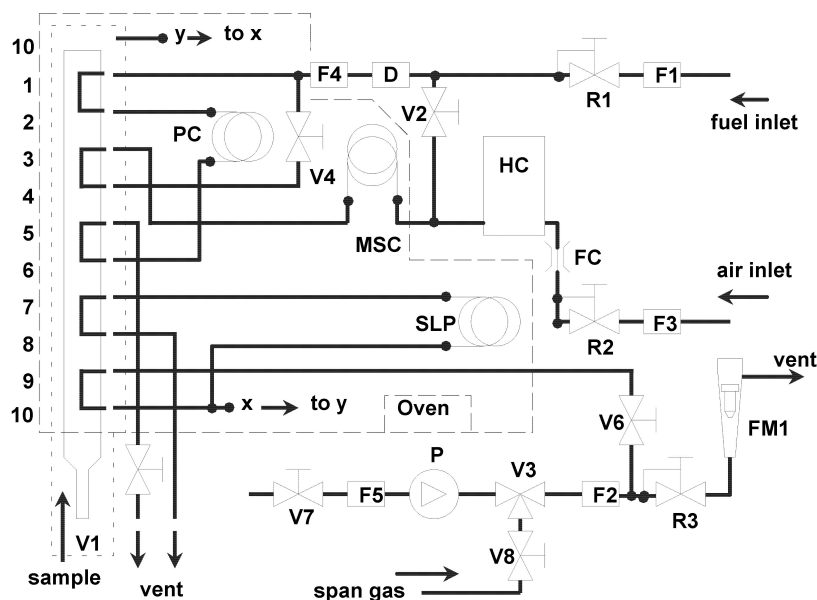
Figure 9: Flow diagram for methane analysis (GC method)
