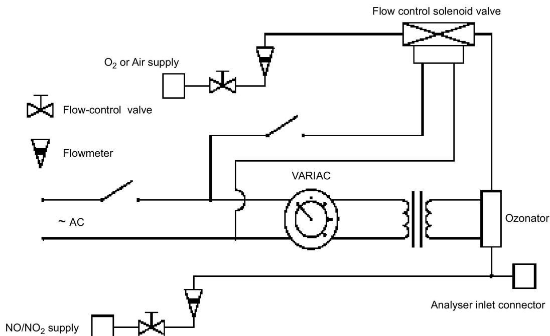
Diagram of NO x converter efficiency devices
