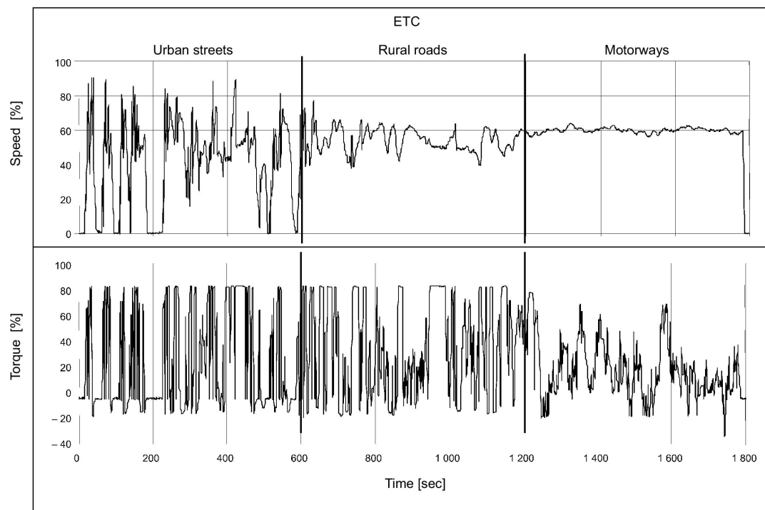
Figure 5: ETC Dynamometer Schedule
