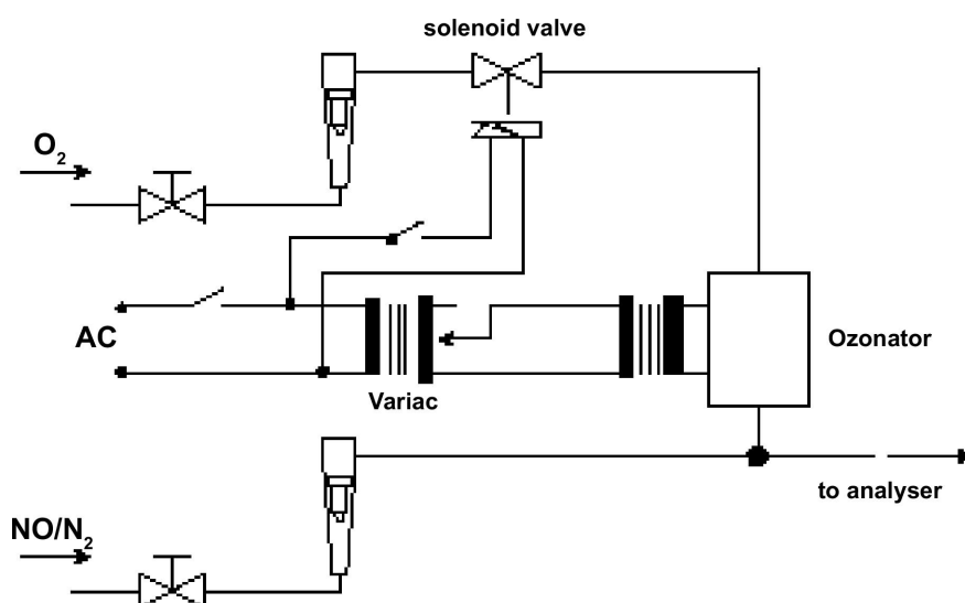
Figure 6: Schematic of NO 2 converter efficiency device
