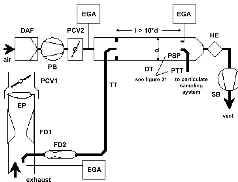
Figure 16: Partial flow dilution system with twin venturi or twin orifice, concentration measurement and fractional sampling
