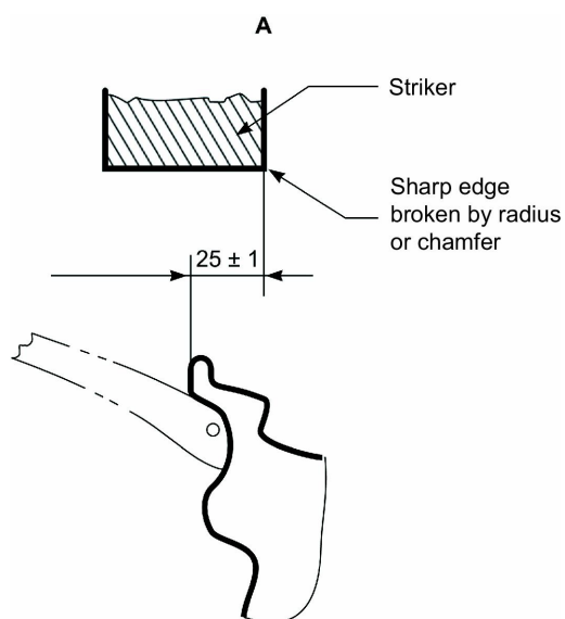
Figure 1 – Detail A
