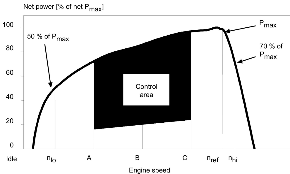
Figure 1: Specific definitions of the test cycles
