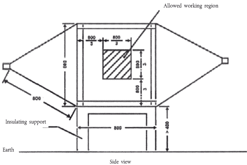
Figure 2 800 mm stripline dimensions
