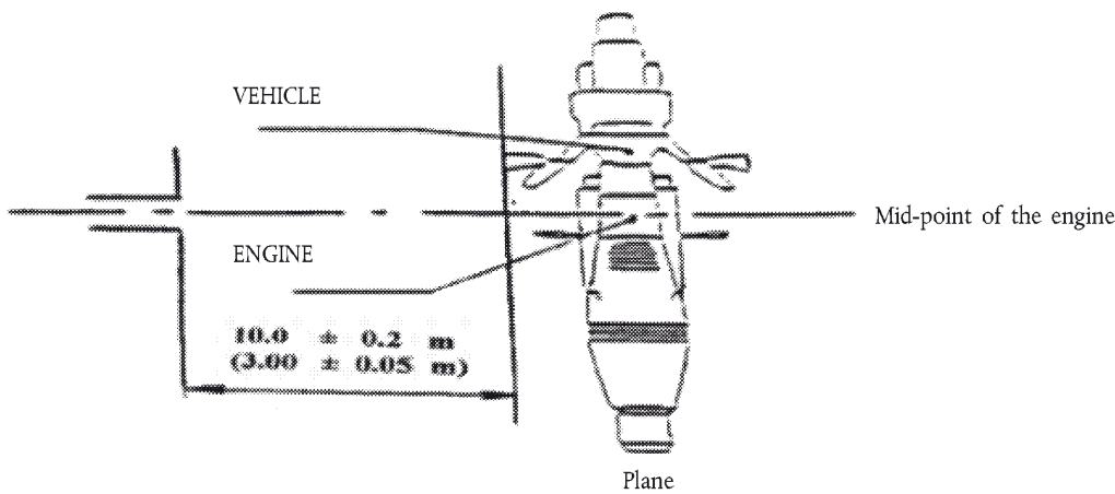
Dipole antenna in position to measure the horizontal radiation components
