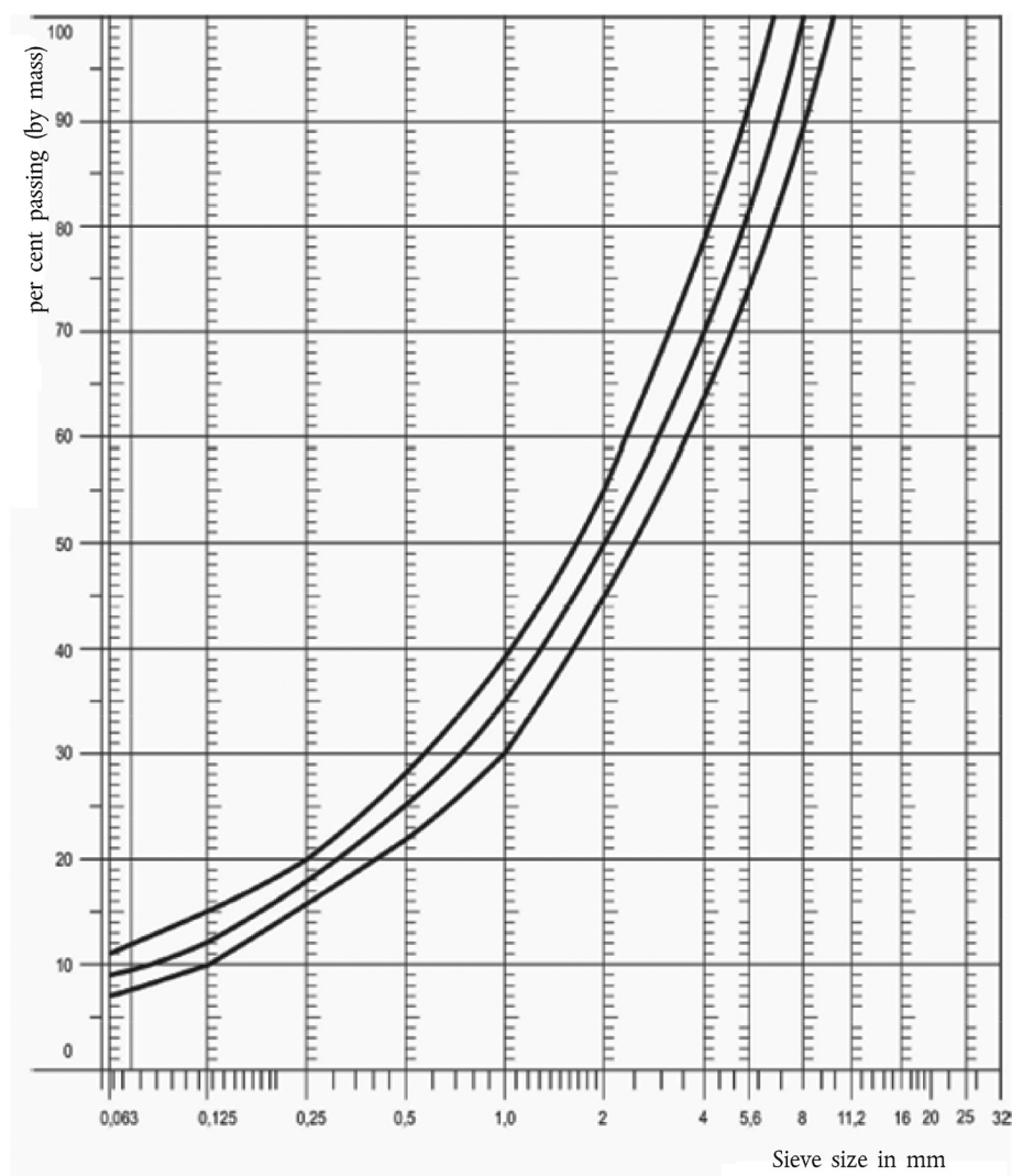
Grading curve of the aggregate in the asphaltic mix with tolerances
