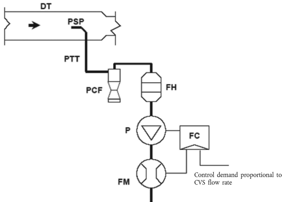
Figure 12 Particulate Sampling System
