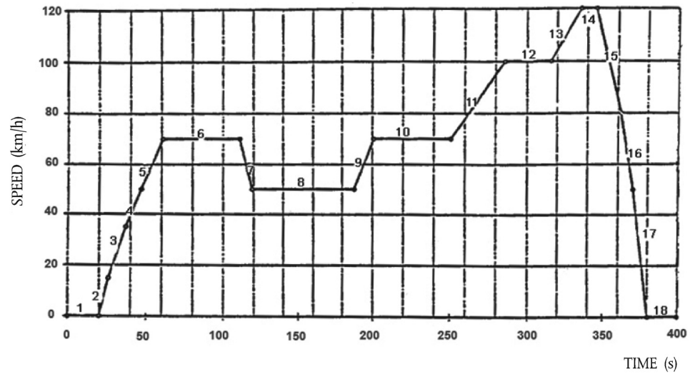
Extra-urban cycle (400 seconds)
