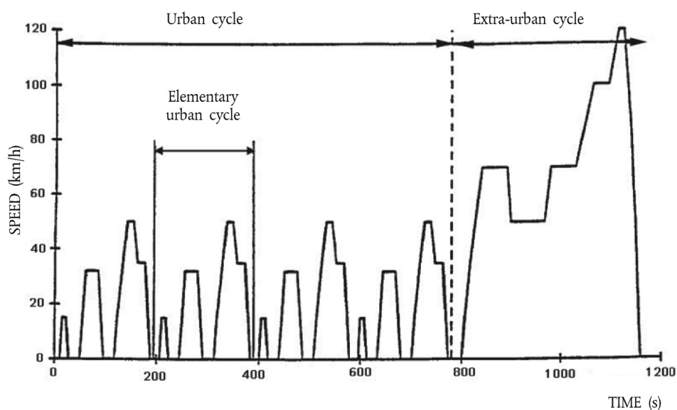
Test sequence — M_1 and N_1 categories of vehicles
