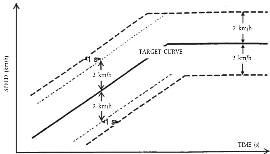
Figure 4 Speed tolerance
