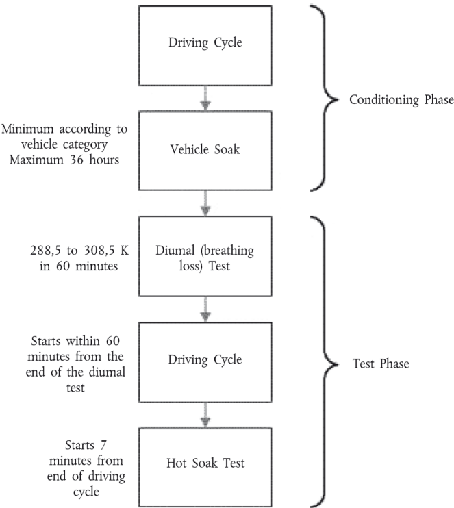
Flow chart – evaporative emission SHED test
