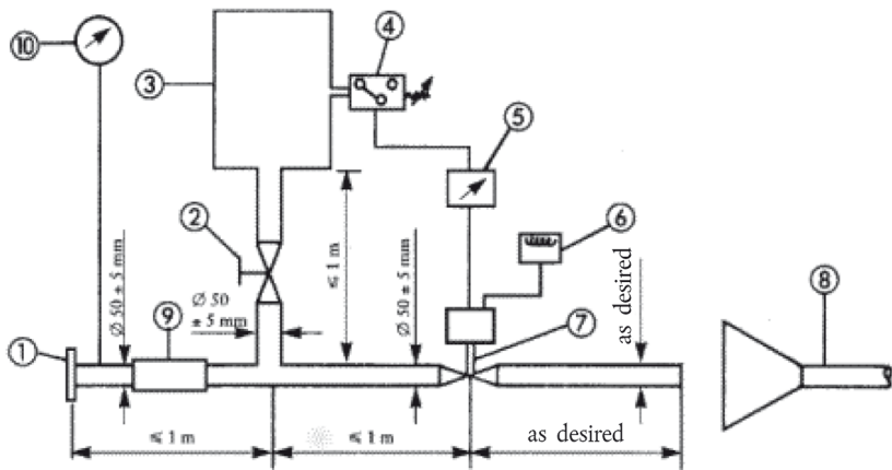
Test apparatus for conditioning by pulsation
