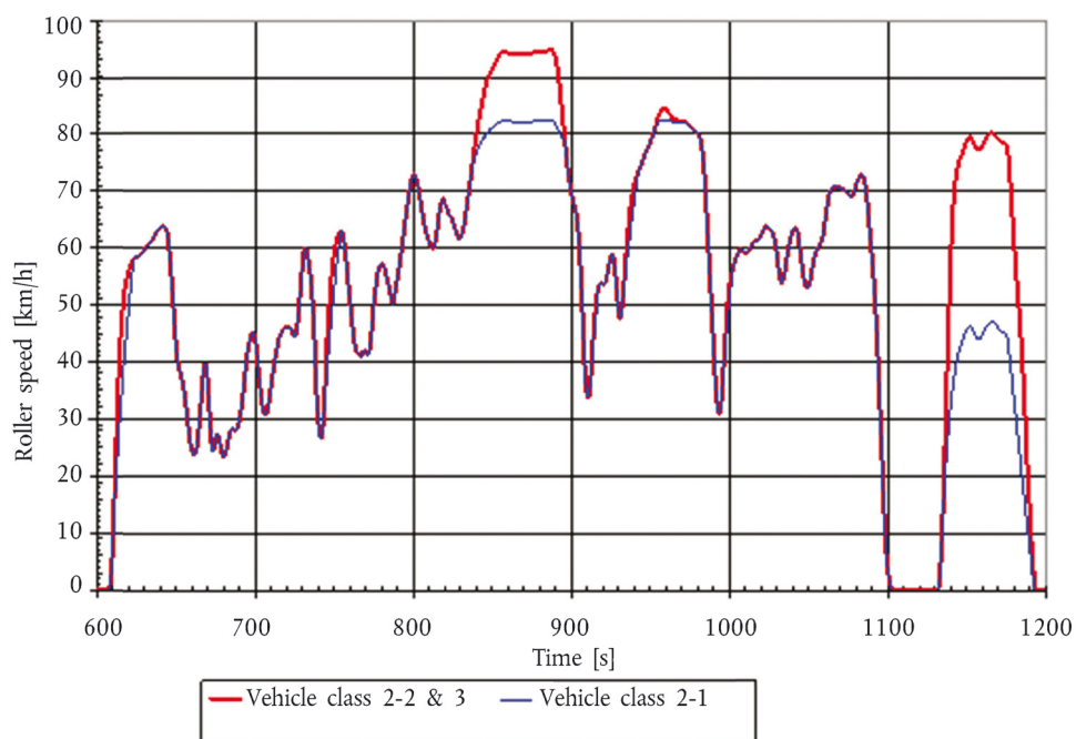
WMTC stage 2, part 2
