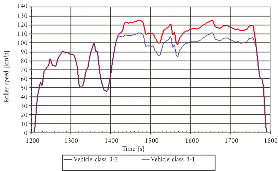
Figure Ap6-8 WMTC stage 2, part 3
