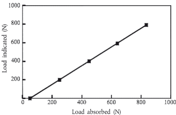
Figure Ap3-2 Load indicated at 80 km/h in terms of load absorbed at 80 km/h
