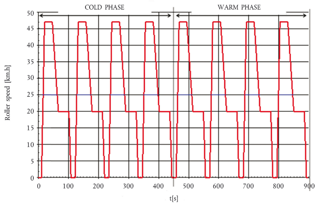
ECE R47-based test cycle
