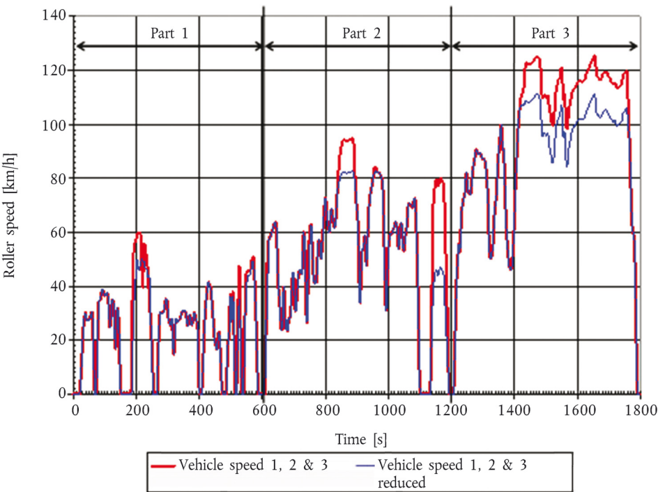
Figure Ap6-5 WMTC stage 2
