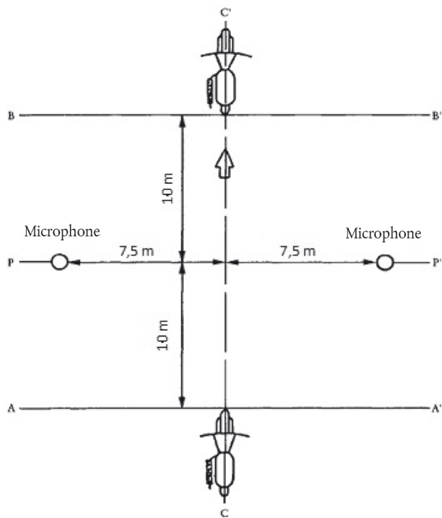
Figure Ap1-2 Test for vehicle in motion
