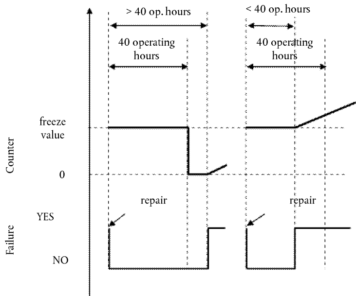
Reactivation and resetting to zero of a counter after a period when its value has been frozen
