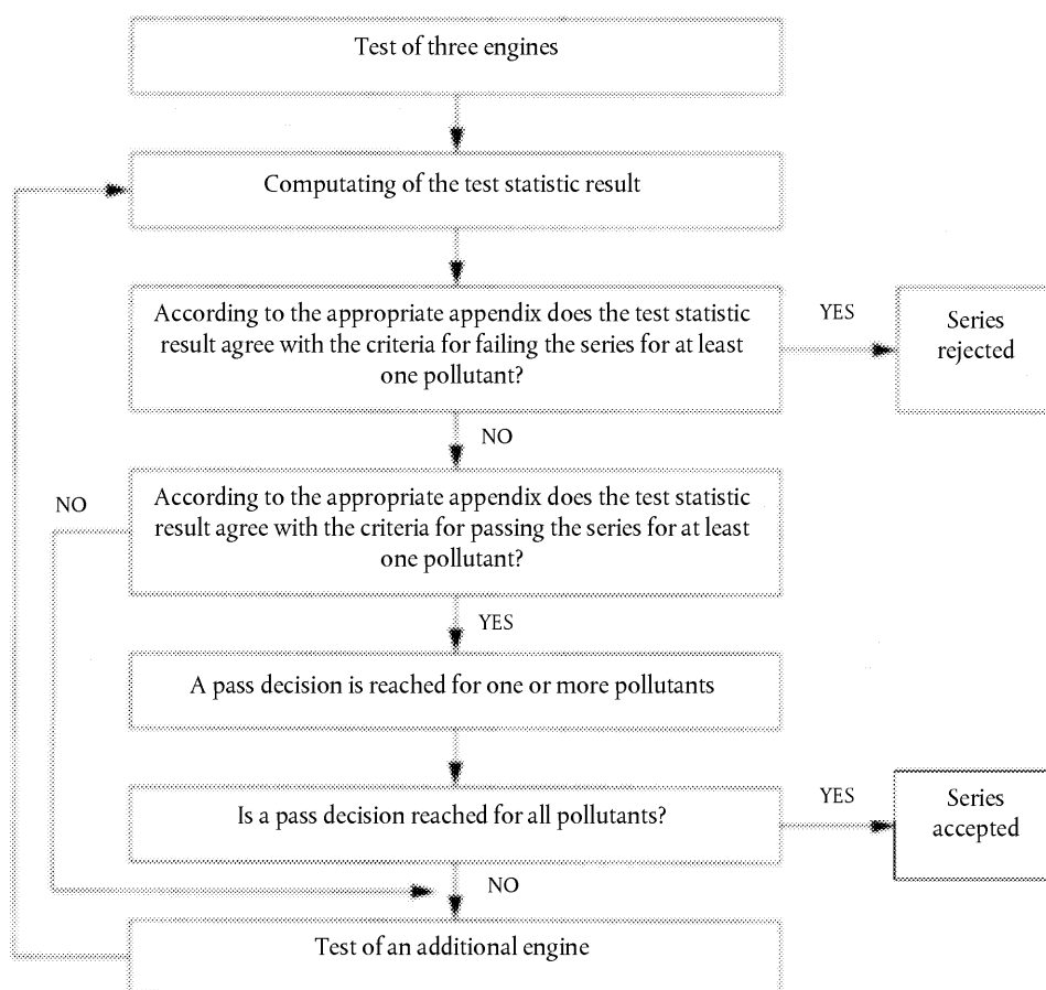
Figure 2.1 Schematic of production conformity testing
