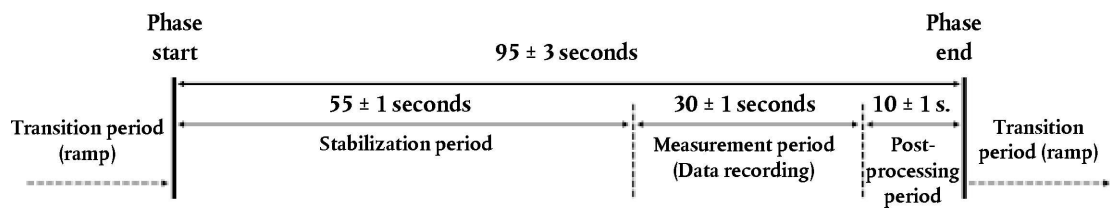
Figure 4 exemplarily illustrates the sequence of steady state measurement setpoints to be followed for the test.
