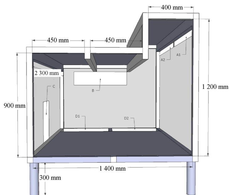
Framework for the test apparatus
