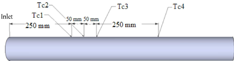
Thermocouples on the exhaust manifold mock-up
