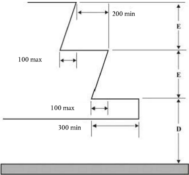
Figure 8 Steps for passengers (dimensions in mm) (see Annex 3, paragraph 7.7.7)
