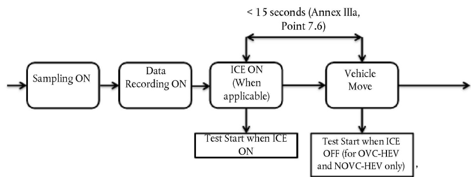
Figure App.1.1 Test Start Sequence
