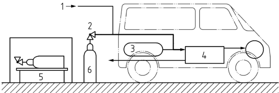
Figure A8.App7/1 Example of instrumentation
