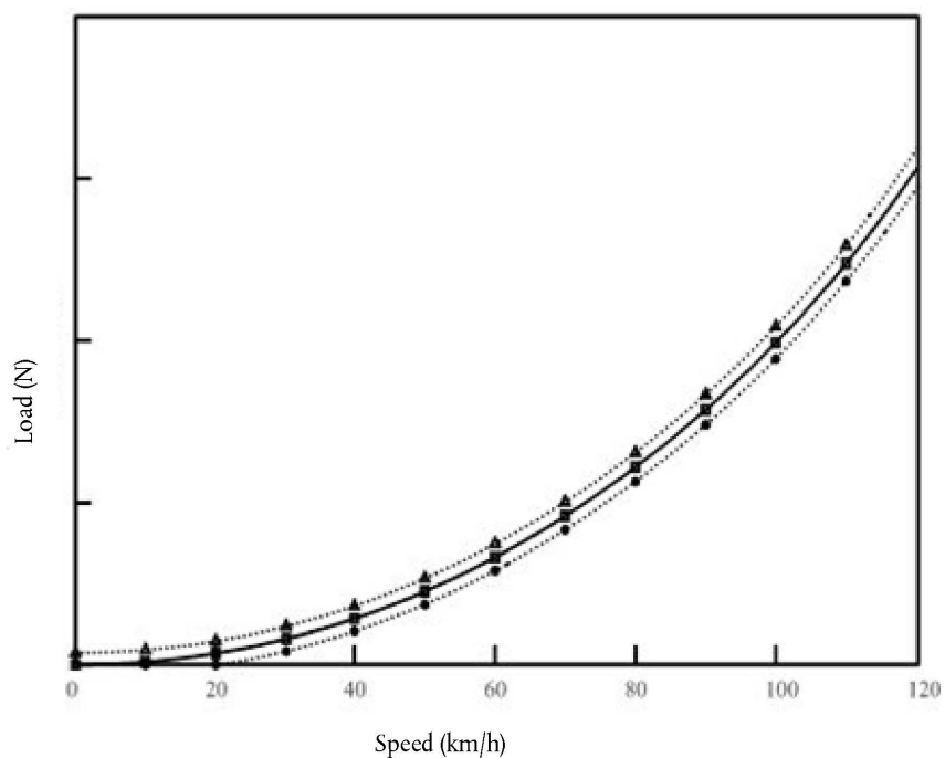
Diagram illustrating the power absorbed by the chassis dynamometer
