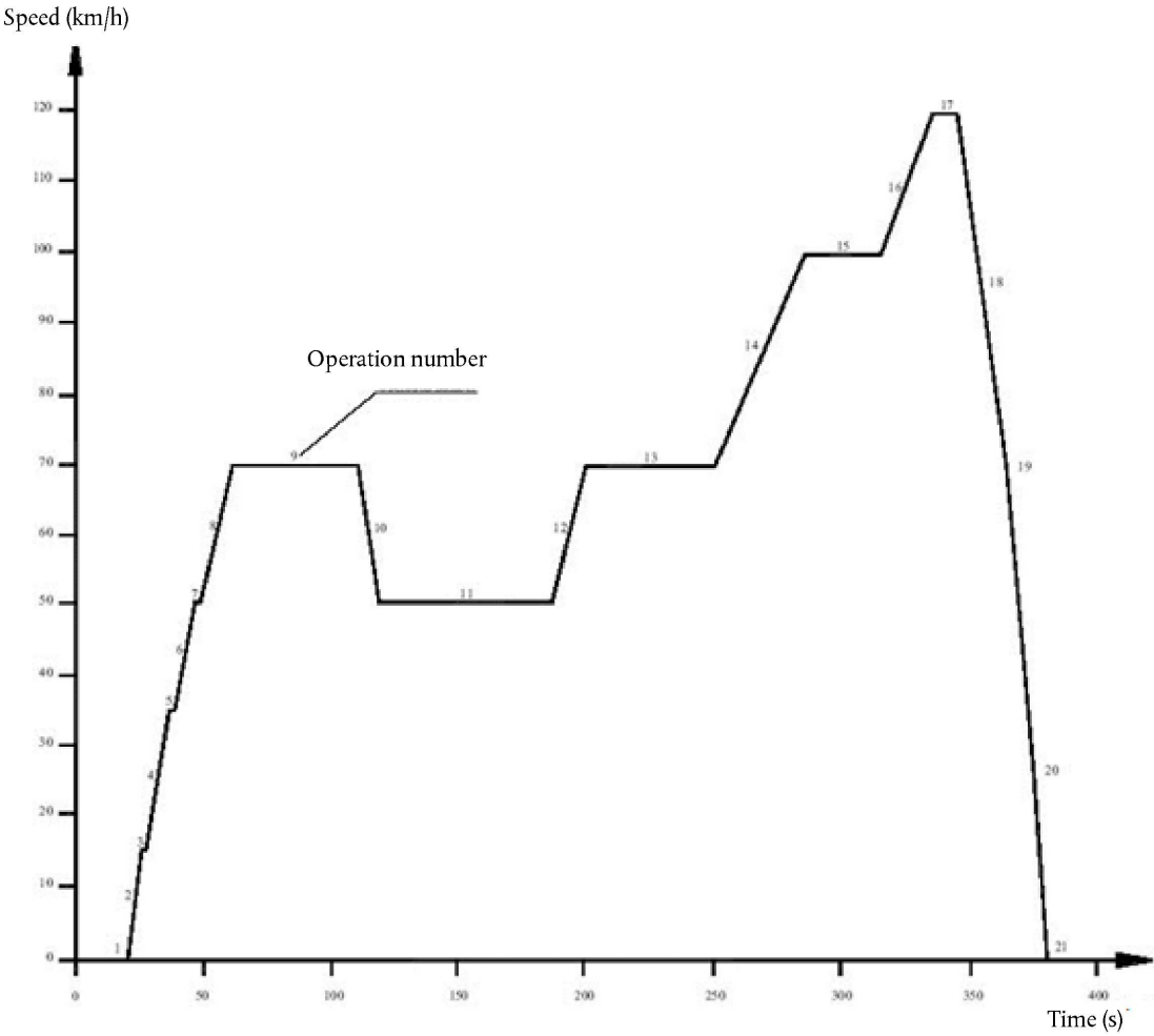
Figure A4a/3 Extra-urban cycle (Part Two) for the Type I test
