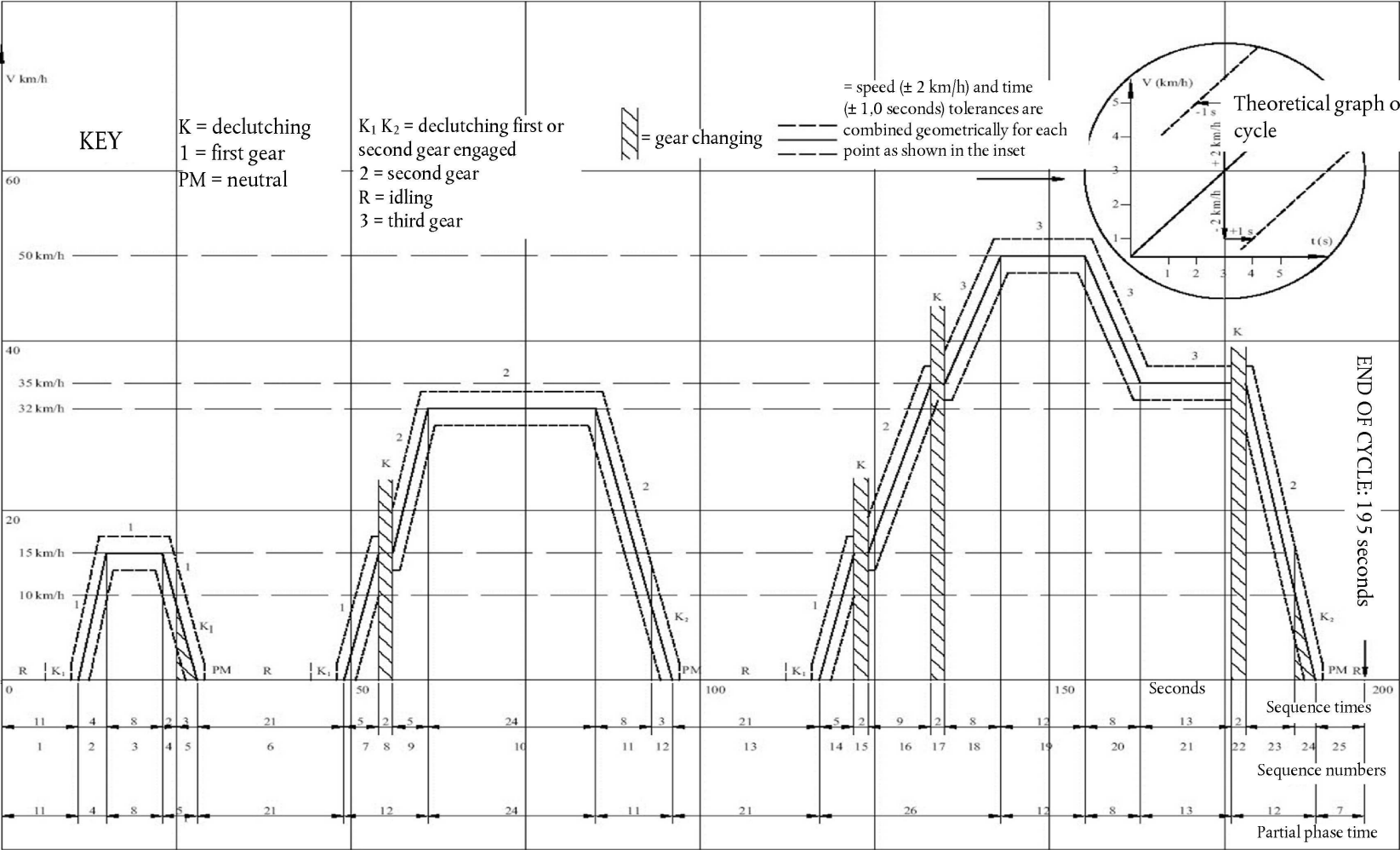
Figure A4a/2 Elementary urban cycle for the Type I test
